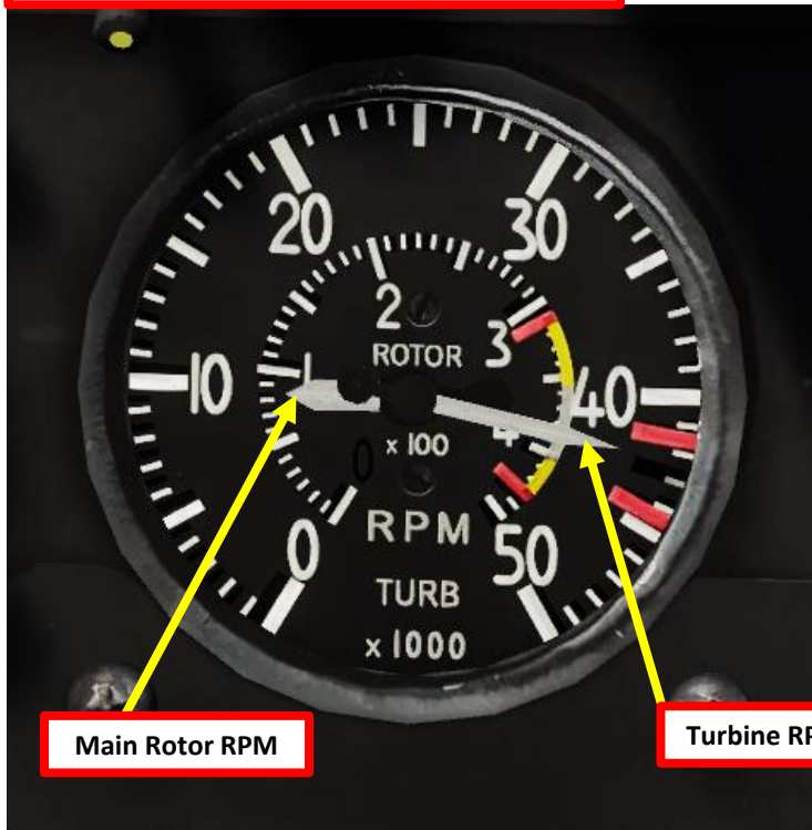
16a Turbine & Main Rotor RPM not Synchronized
