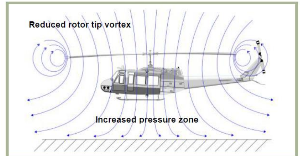
Airflow when In Ground Effect (IGE) (UH-1H)
