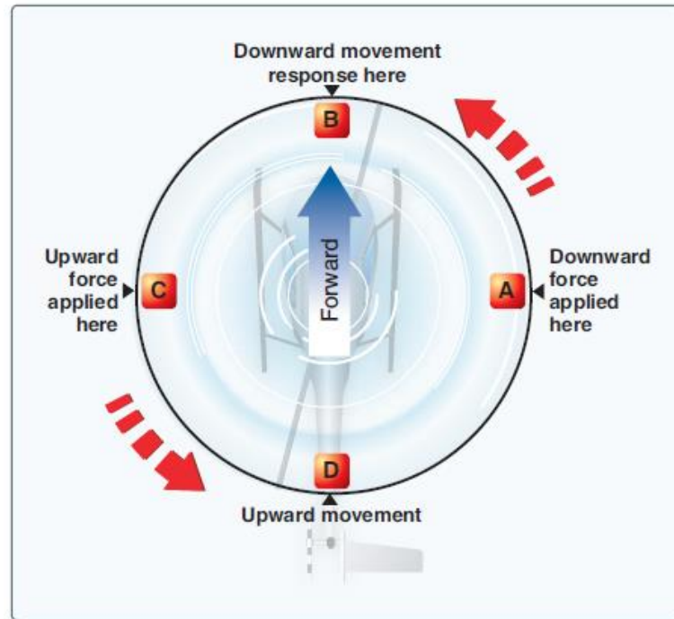
Gyroscopic Precession
