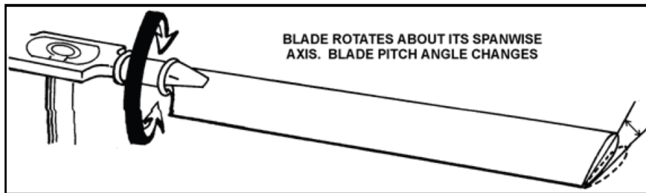
Figure 1-17. Feathering
