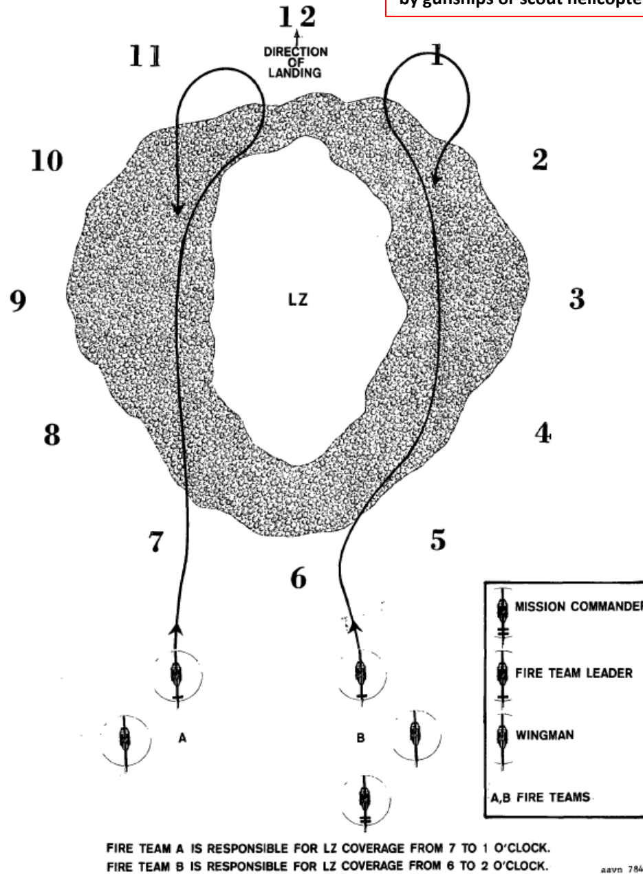
Figure 26. Double orbit of the landing zone.
